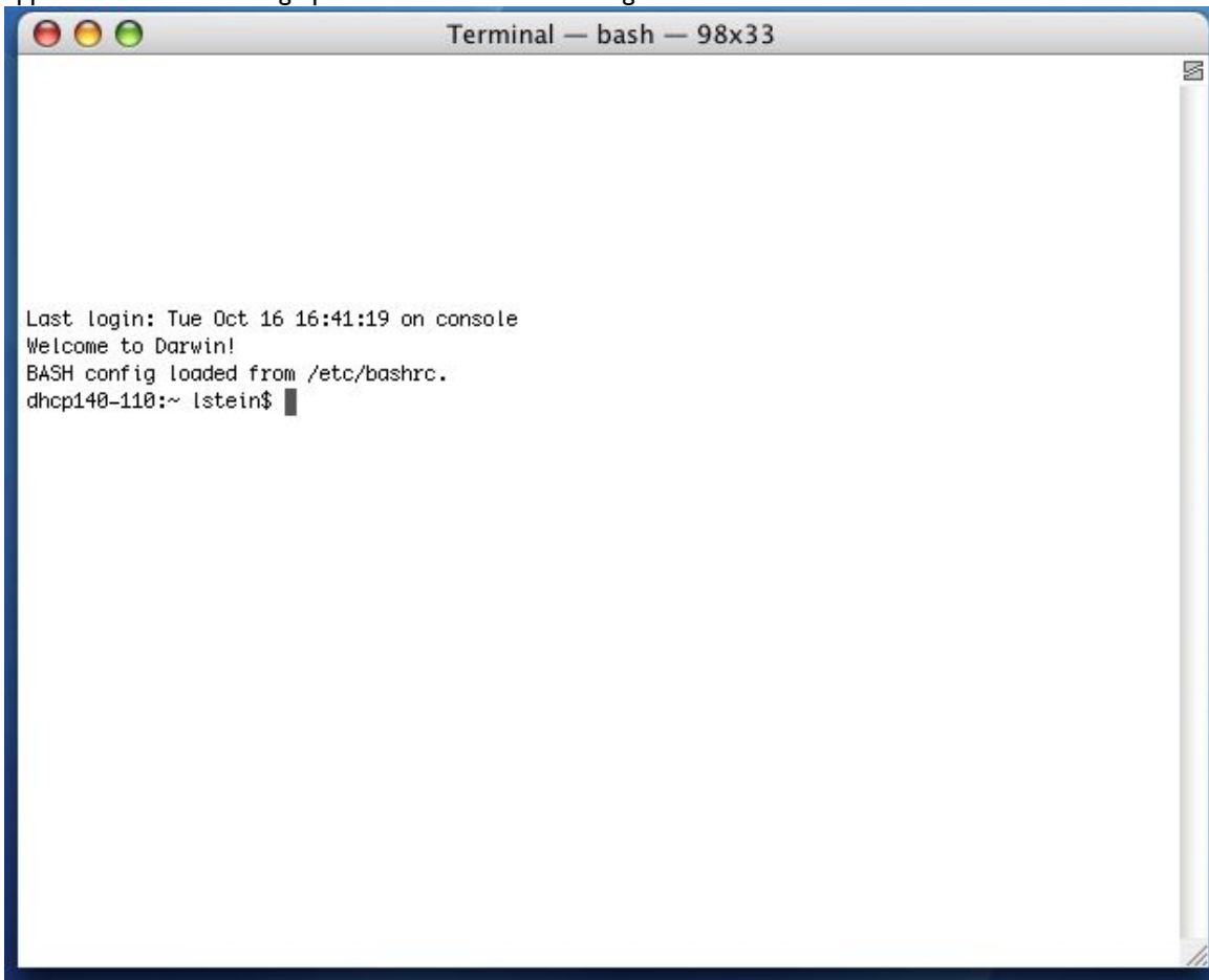
OSX Terminal
